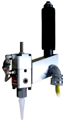
2600-084-000 Electric Handle (Shown With 2600-041 Valve)
